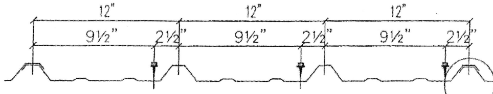
MEMBER SCREW LOCATION DETAIL "A" (ALL MEMBERS EXCEPT AS NOTED)
