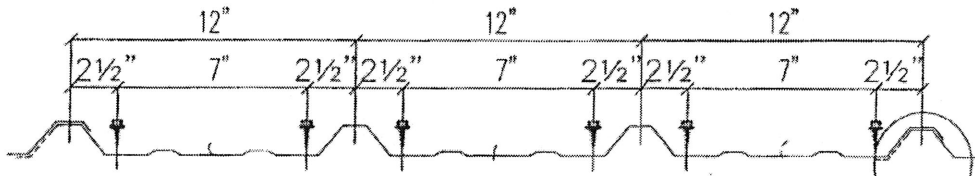
MEMBER SCREW LOCATION DETAIL "A" (PEAK PURLIN, EAVE STRUT, AND PANEL END LAPS)
